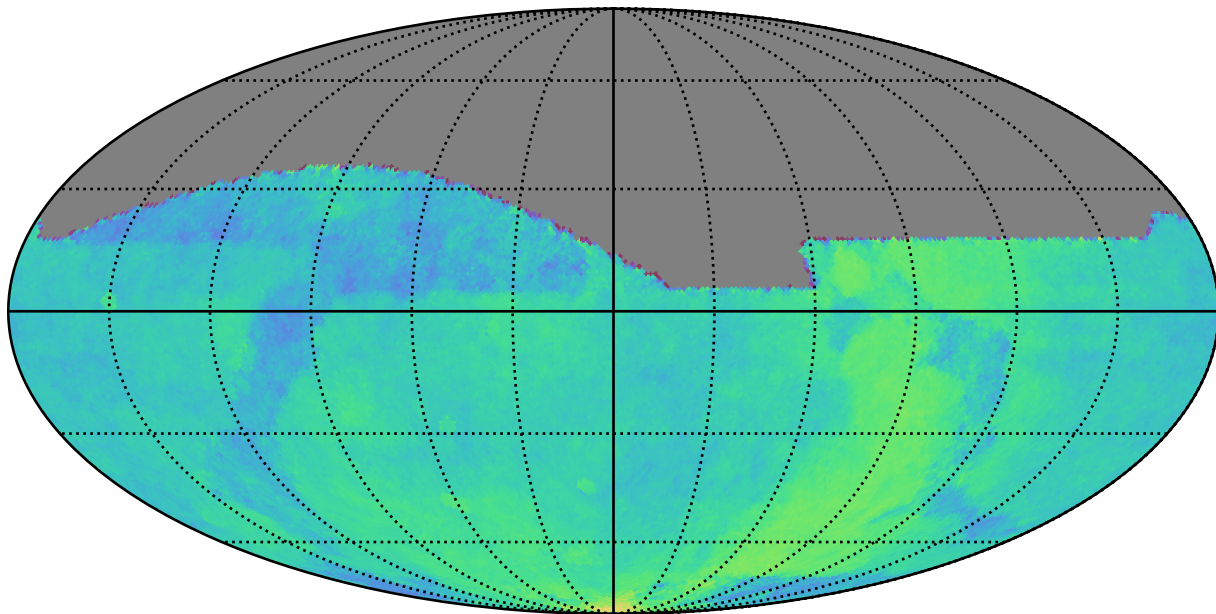
too_elab_r16_d3_gz_v3.4_10yrs All sky: Parallax Coverage @ 22.4
