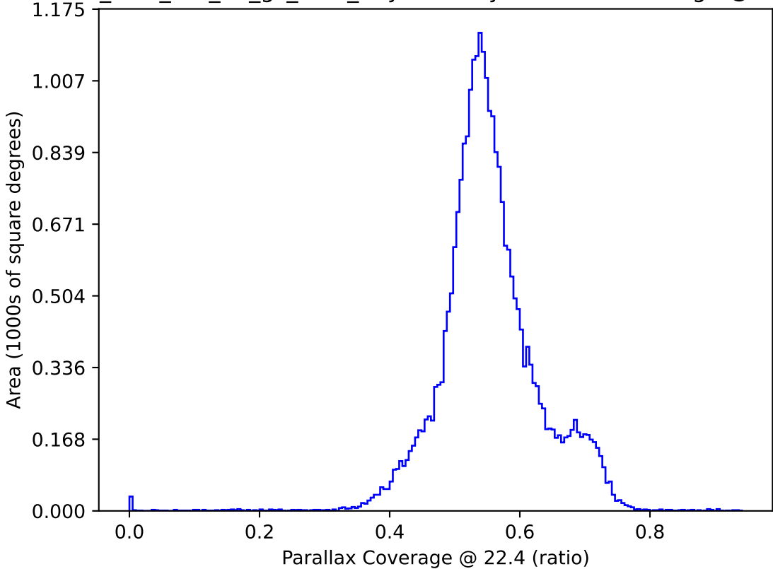
too_elab_r16_d3_gz_v3.4_10yrs All sky: Parallax Coverage @ 22.4
