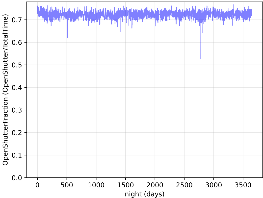
too_elab_r16_d3_gz_v3.4_10yrs Per night: OpenShutterFraction
