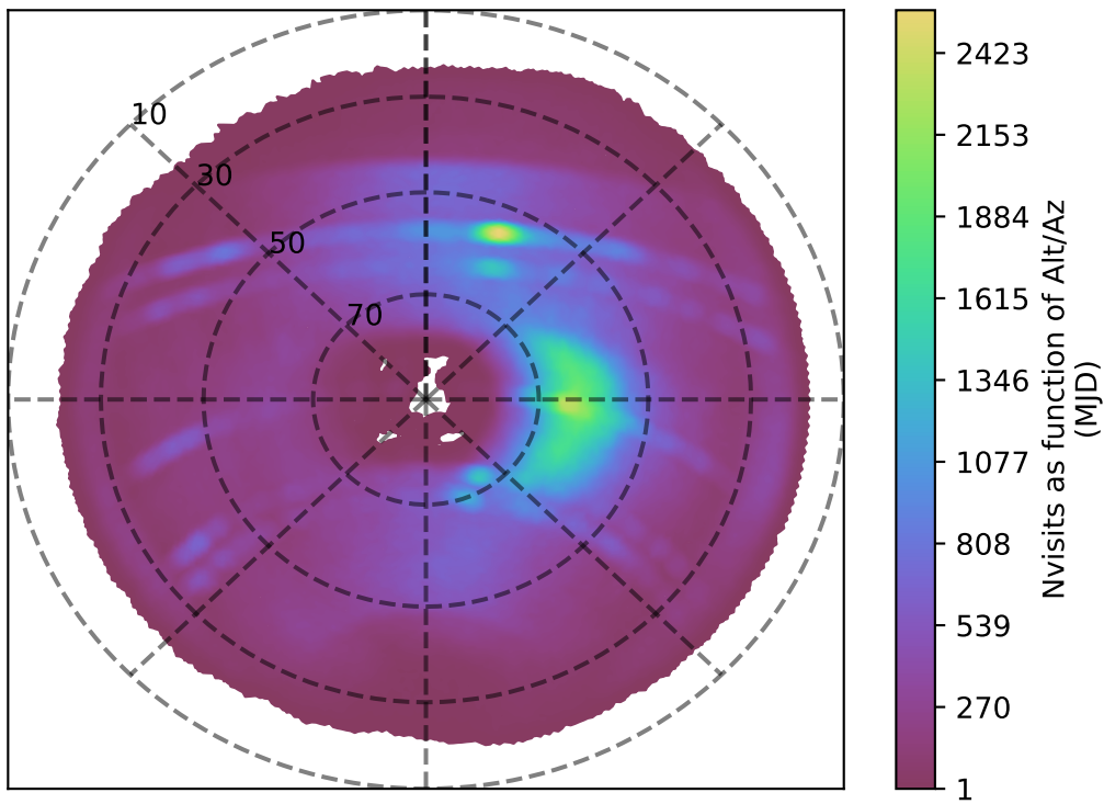
too_elab_r16_d3_gz_v3.4_10yrs z band: Nvisits as function of Alt/Az
