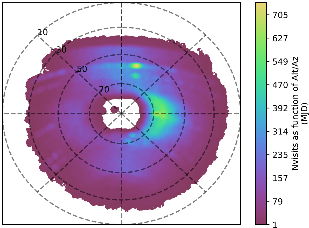
too_elab_r16_d3_gz_v3.4_10yrs u band: Nvisits as function of Alt/Az
