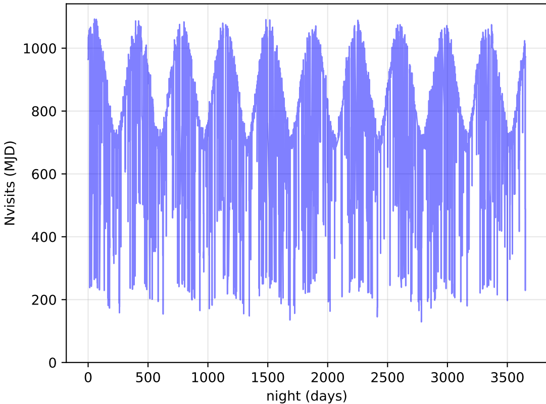
too_elab_r16_d3_gz_v3.4_10yrs All visits: Nvisits
