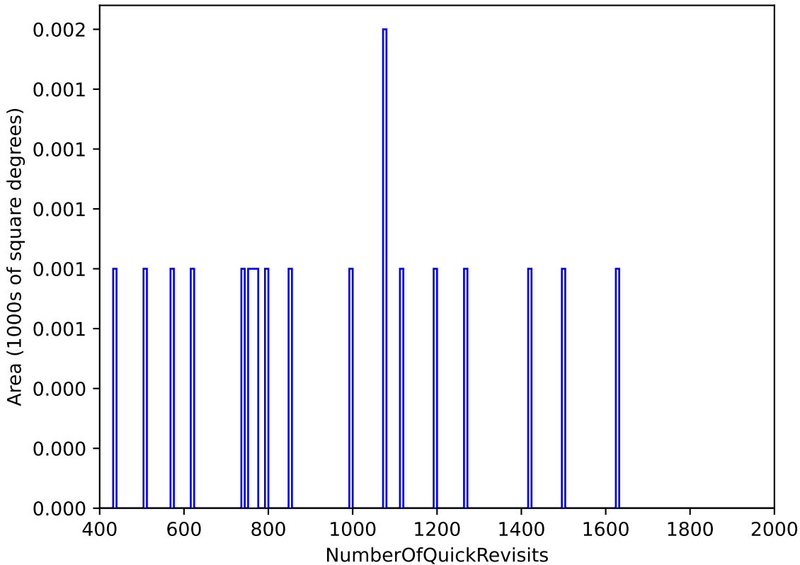
too_elab_r16_d3_gz_v3.4_10yrs All sky: NumberOfQuickRevisits
