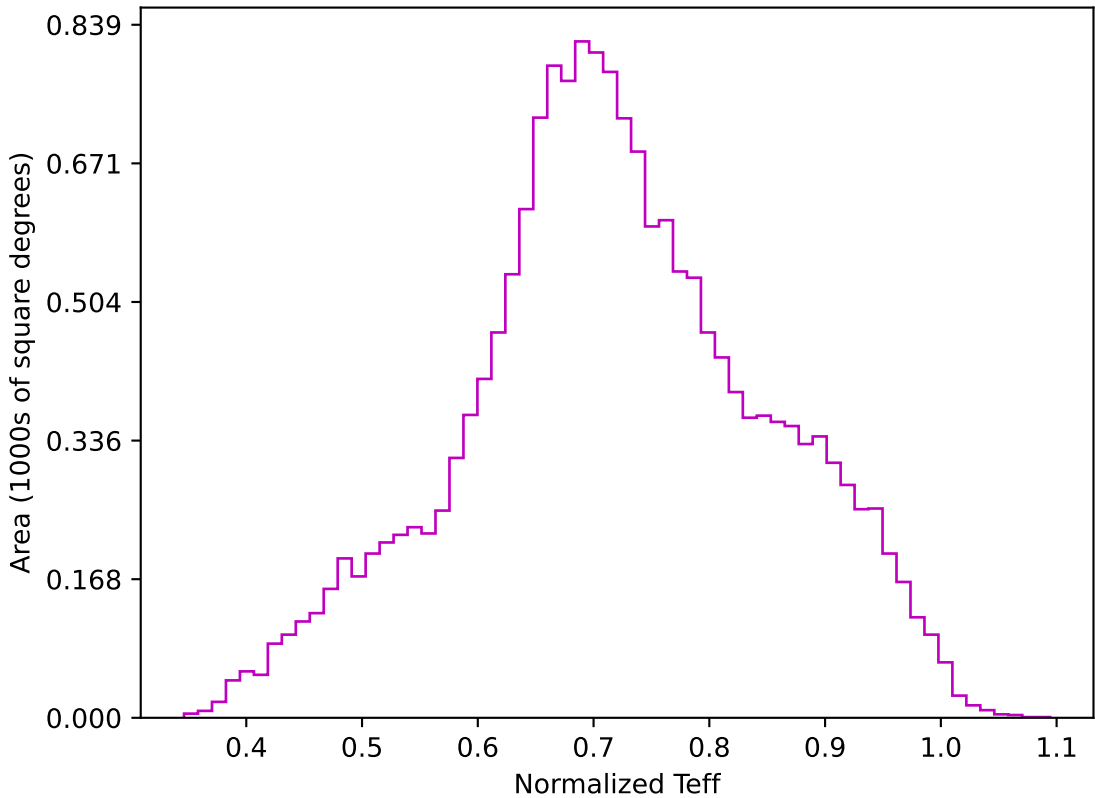
too_elab_r16_d3_gz_v3.4_10yrs WFD z band: Normalized Teff
