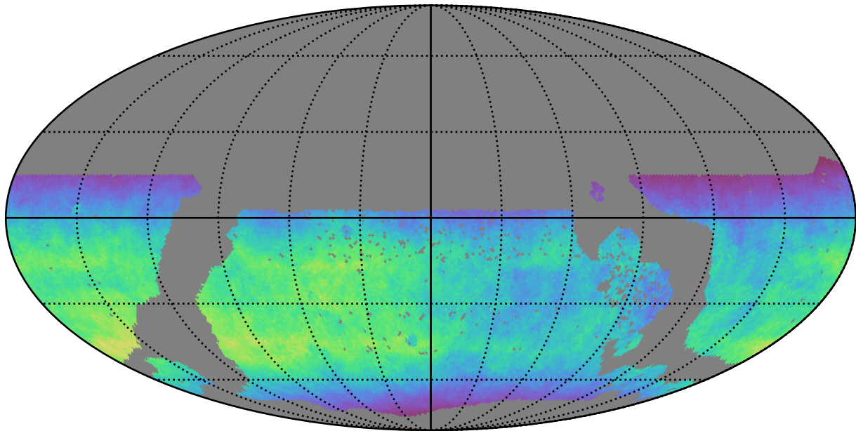
too_elab_r16_d3_gz_v3.4_10yrs WFD y band: Normalized Teff
