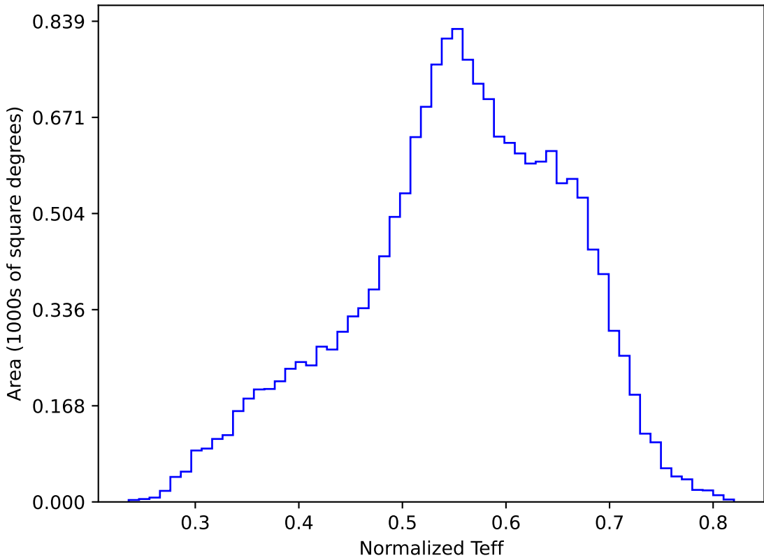
too_elab_r16_d3_gz_v3.4_10yrs WFD y band: Normalized Teff
