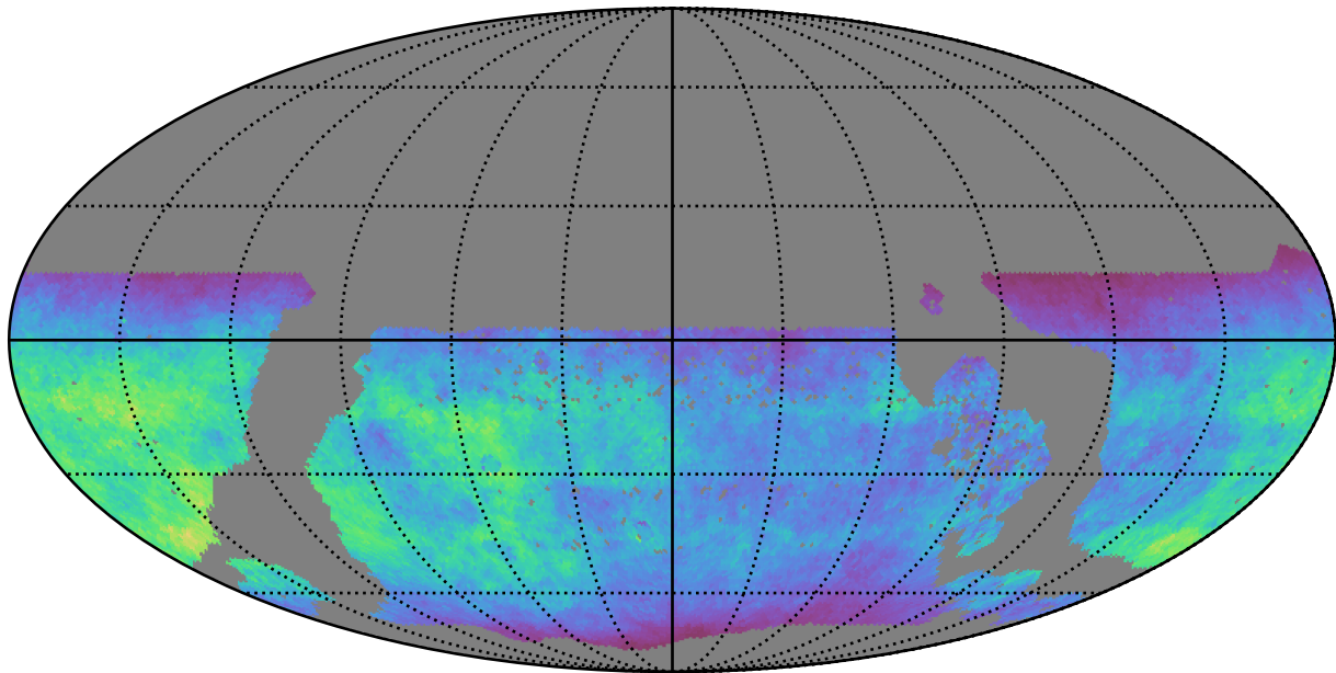
too_elab_r16_d3_gz_v3.4_10yrs WFD u band: Normalized Teff
