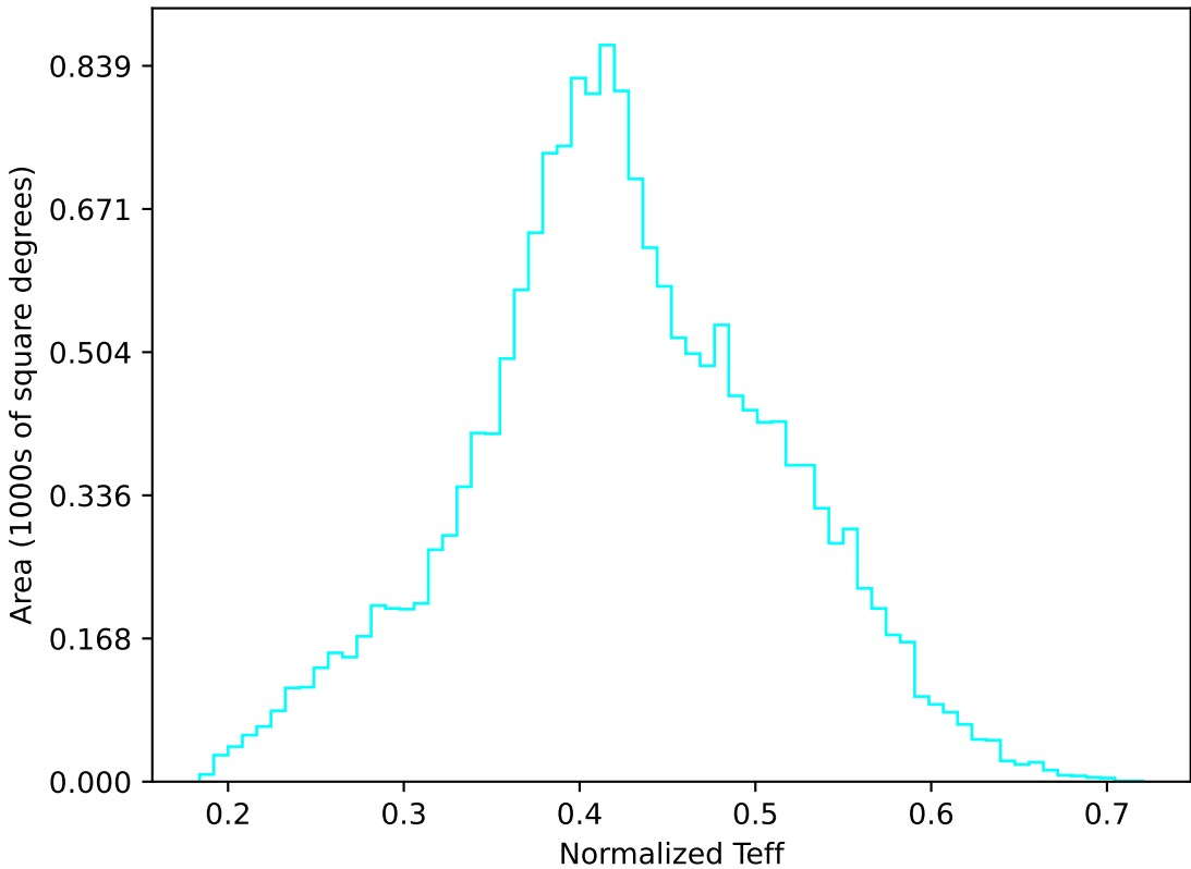
too_elab_r16_d3_gz_v3.4_10yrs WFD u band: Normalized Teff
