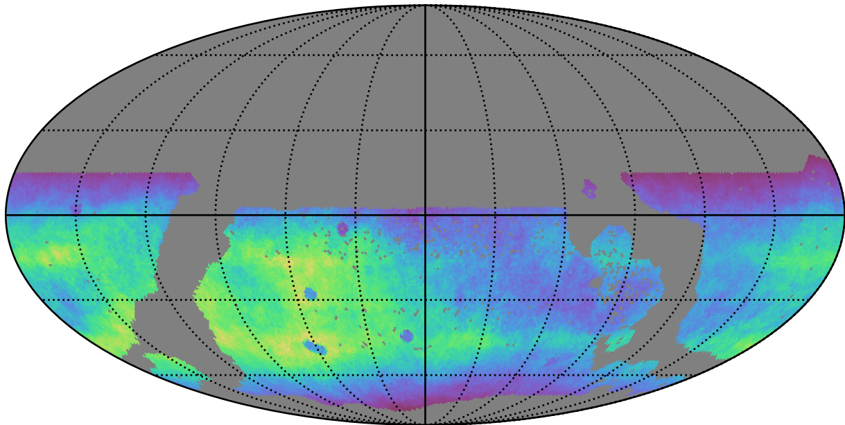
too_elab_r16_d3_gz_v3.4_10yrs WFD r band: Normalized Teff
