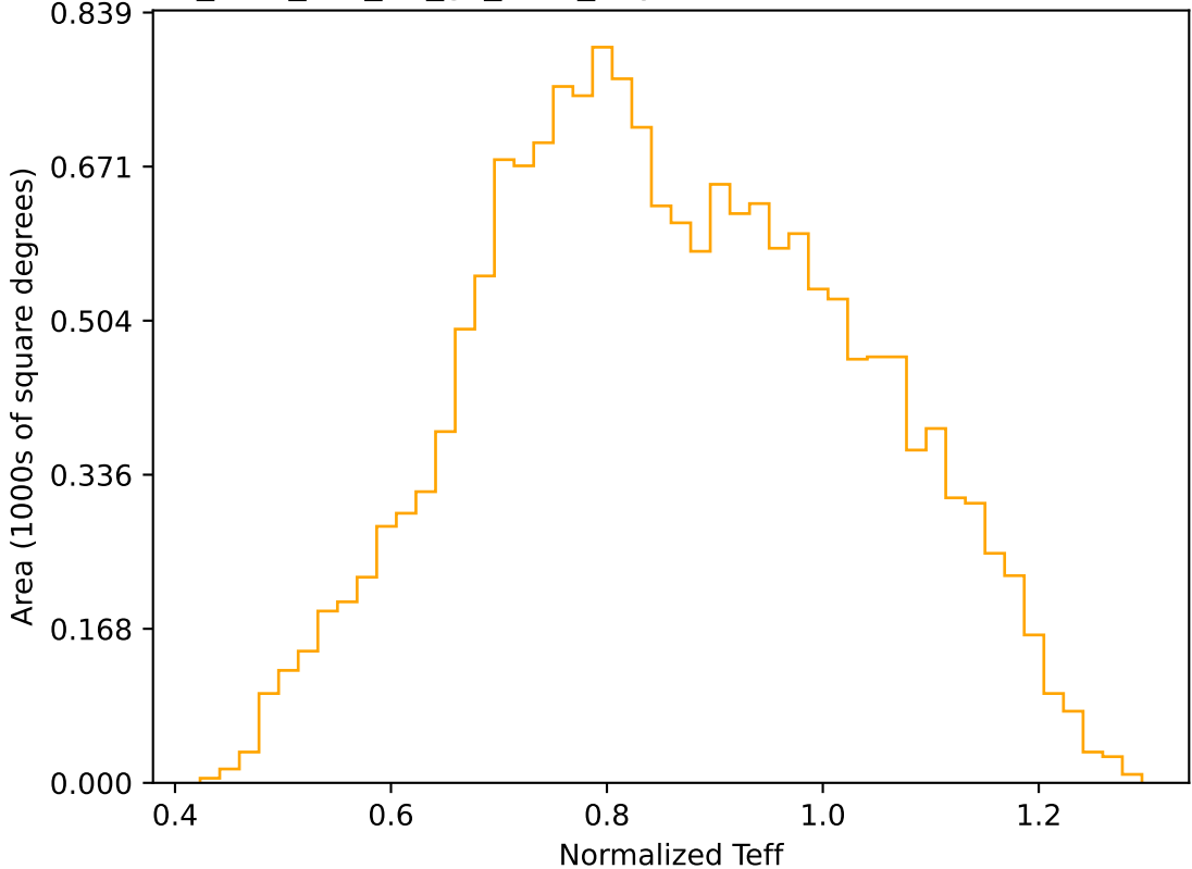
too_elab_r16_d3_gz_v3.4_10yrs WFD r band: Normalized Teff
