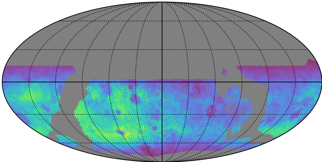
too_elab_r16_d3_gz_v3.4_10yrs WFD g band: Normalized Teff
