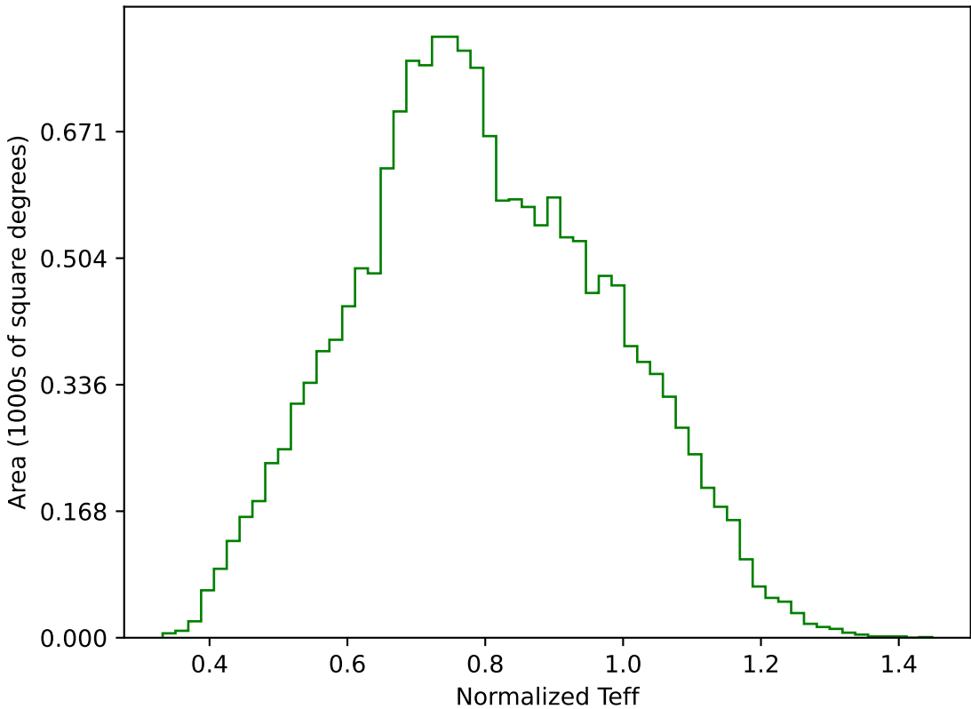
too_elab_r16_d3_gz_v3.4_10yrs WFD g band: Normalized Teff
