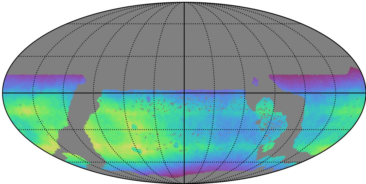
too_elab_r16_d3_gz_v3.4_10yrs WFD all bands: Normalized Teff
