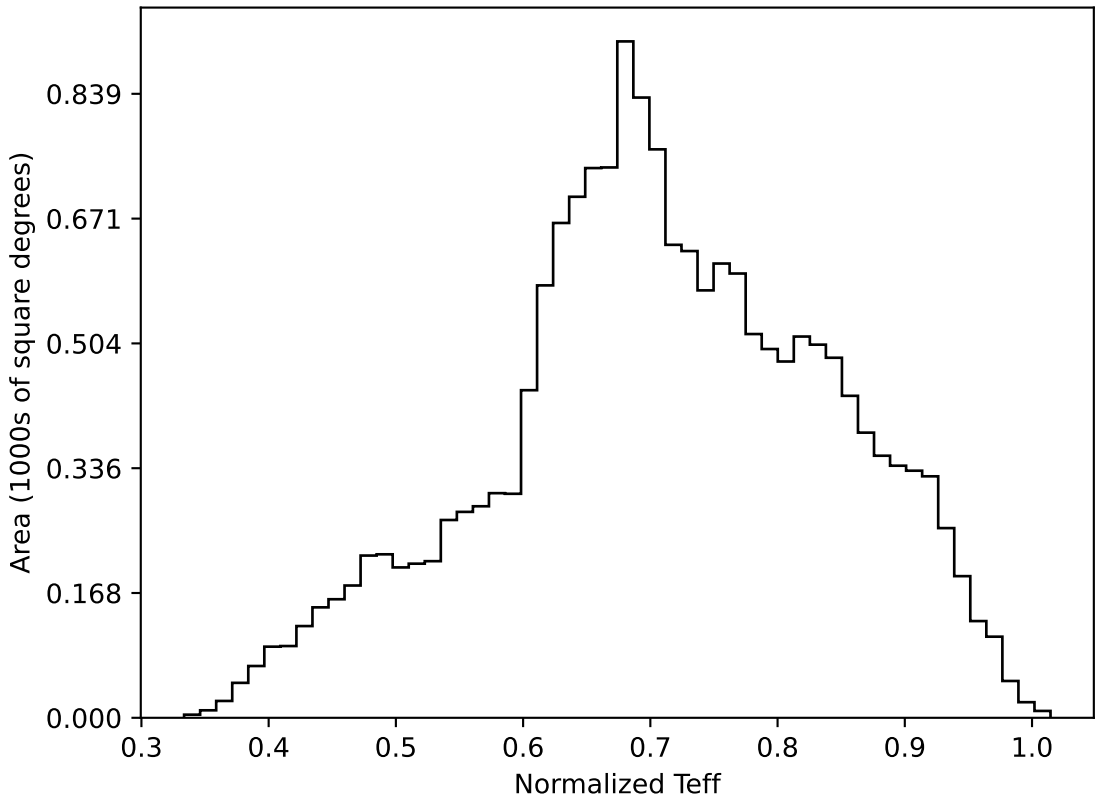
too_elab_r16_d3_gz_v3.4_10yrs WFD all bands: Normalized Teff
