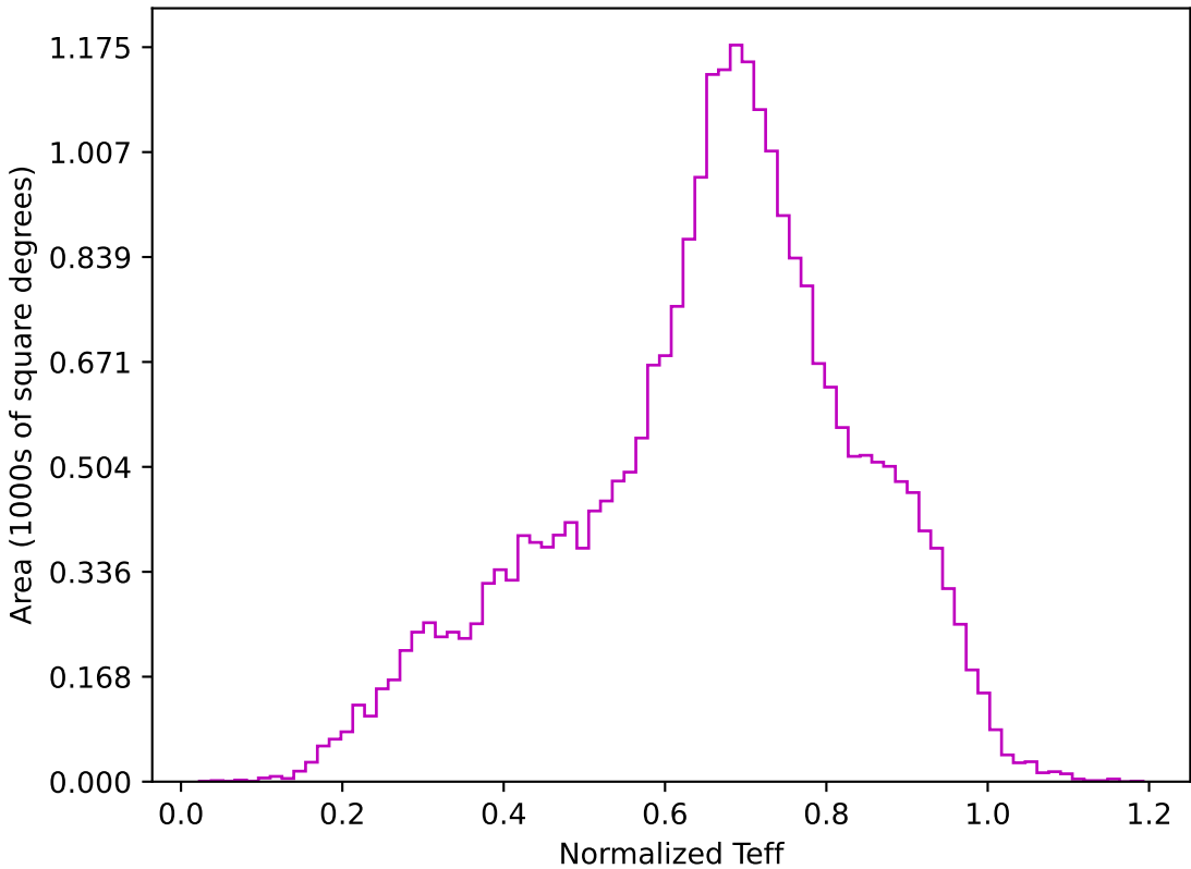
too_elab_r16_d3_gz_v3.4_10yrs All sky z band: Normalized Teff
