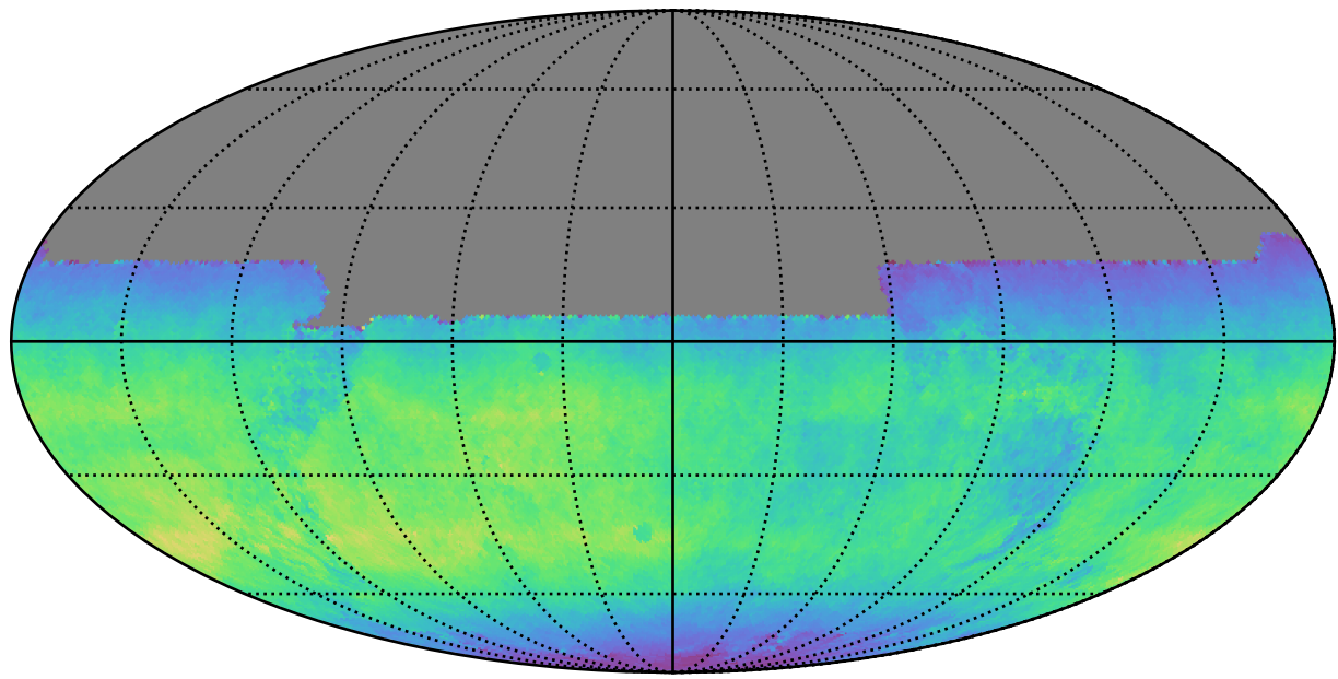
too_elab_r16_d3_gz_v3.4_10yrs All sky y band: Normalized Teff
