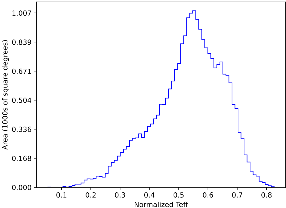
too_elab_r16_d3_gz_v3.4_10yrs All sky y band: Normalized Teff
