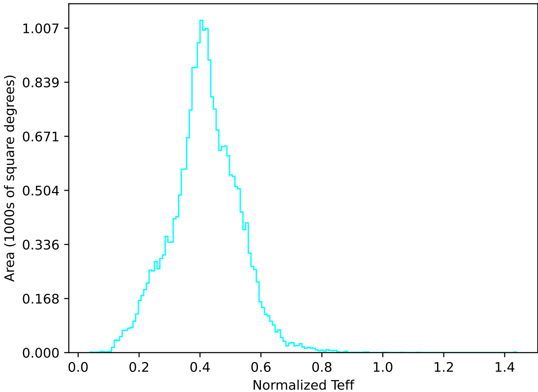
too_elab_r16_d3_gz_v3.4_10yrs All sky u band: Normalized Teff
