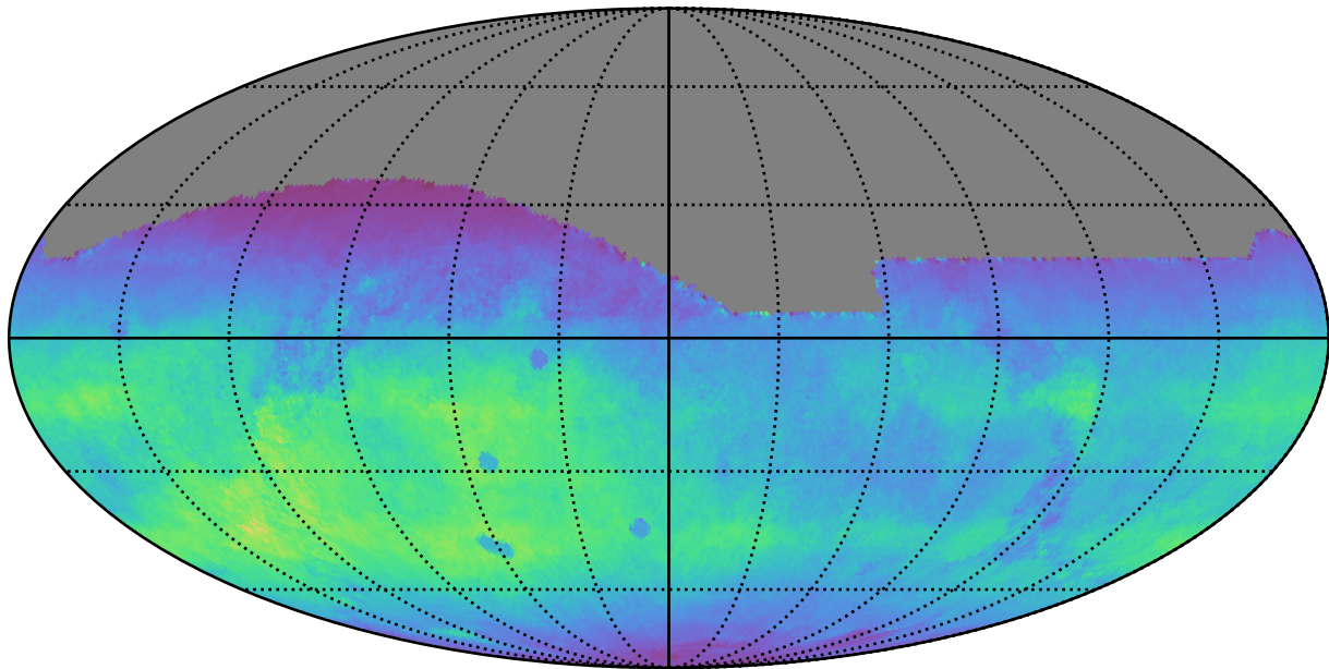
too_elab_r16_d3_gz_v3.4_10yrs All sky r band: Normalized Teff
