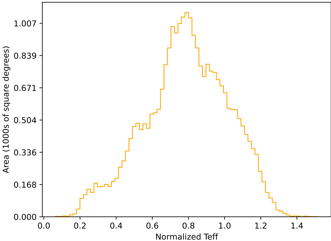
too_elab_r16_d3_gz_v3.4_10yrs All sky r band: Normalized Teff
