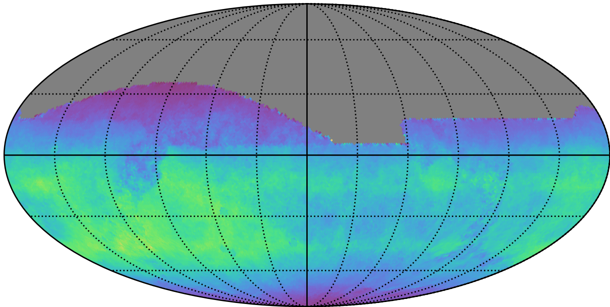
too_elab_r16_d3_gz_v3.4_10yrs All sky i band: Normalized Teff
