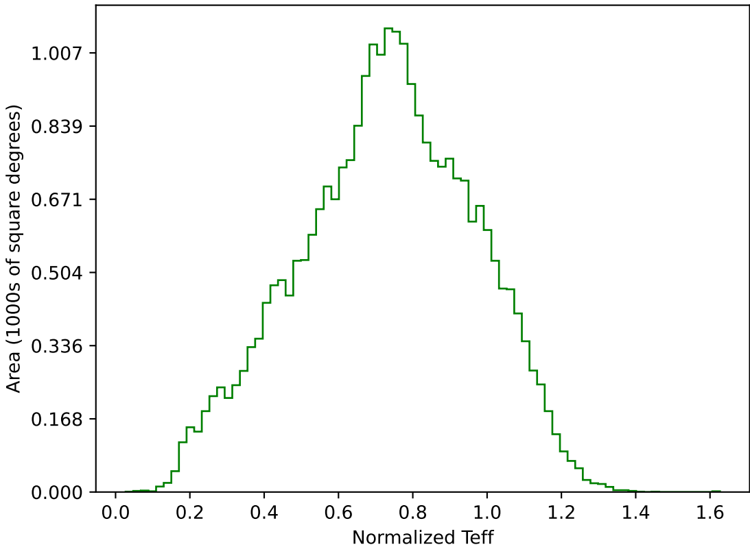
too_elab_r16_d3_gz_v3.4_10yrs All sky g band: Normalized Teff
