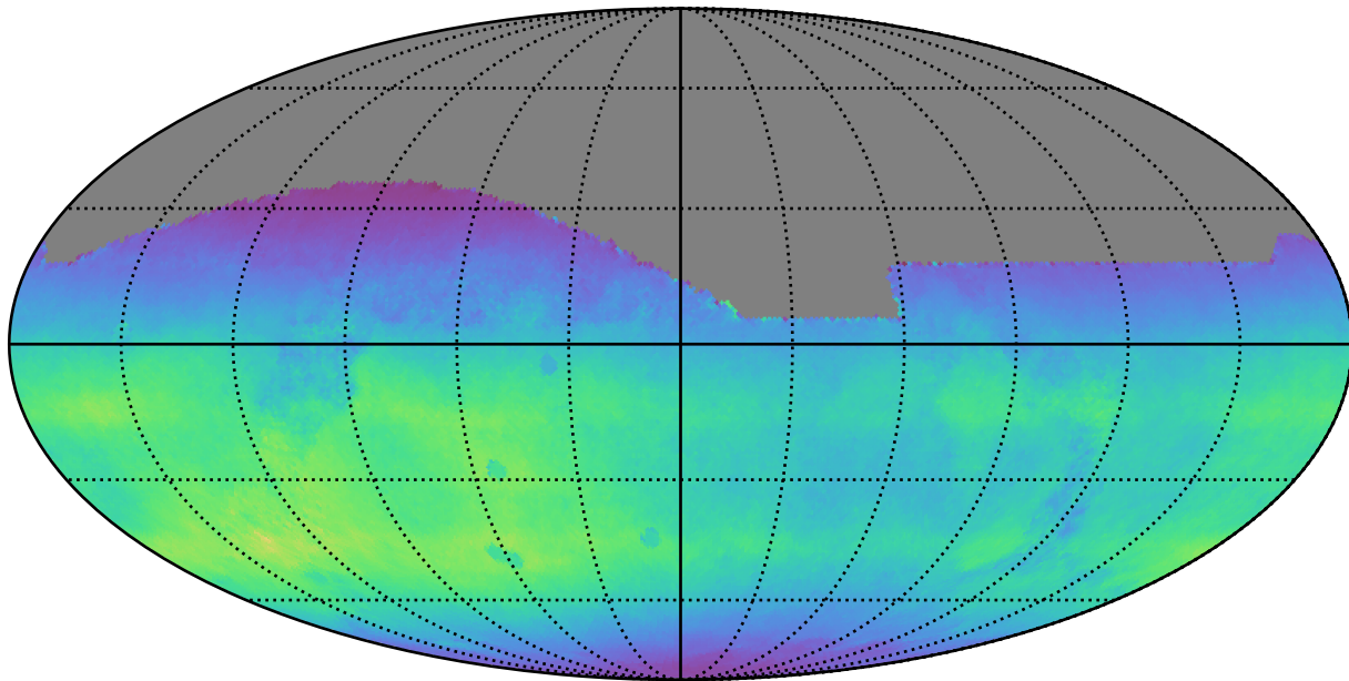
too_elab_r16_d3_gz_v3.4_10yrs All sky all bands: Normalized Teff
