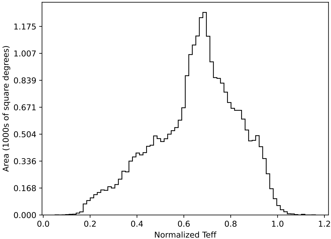
too_elab_r16_d3_gz_v3.4_10yrs All sky all bands: Normalized Teff
