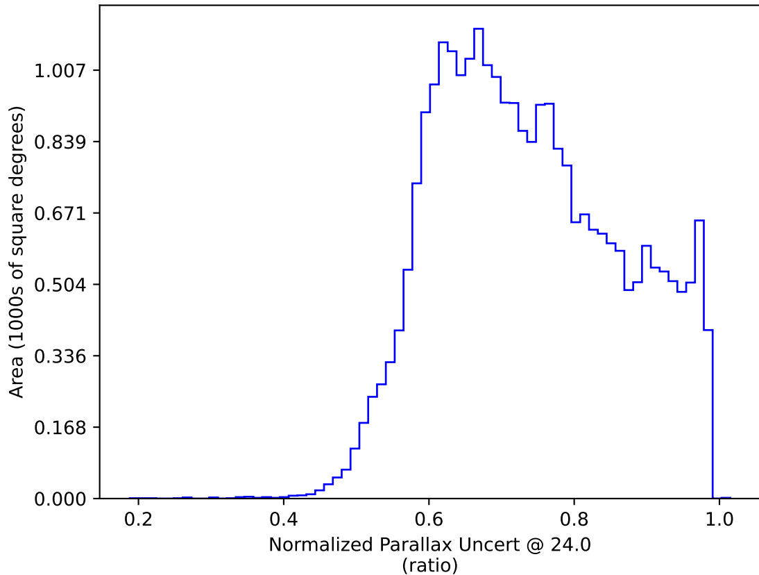
too_elab_r16_d3_gz_v3.4_10yrs All sky: Normalized Parallax Uncert @ 24.0
