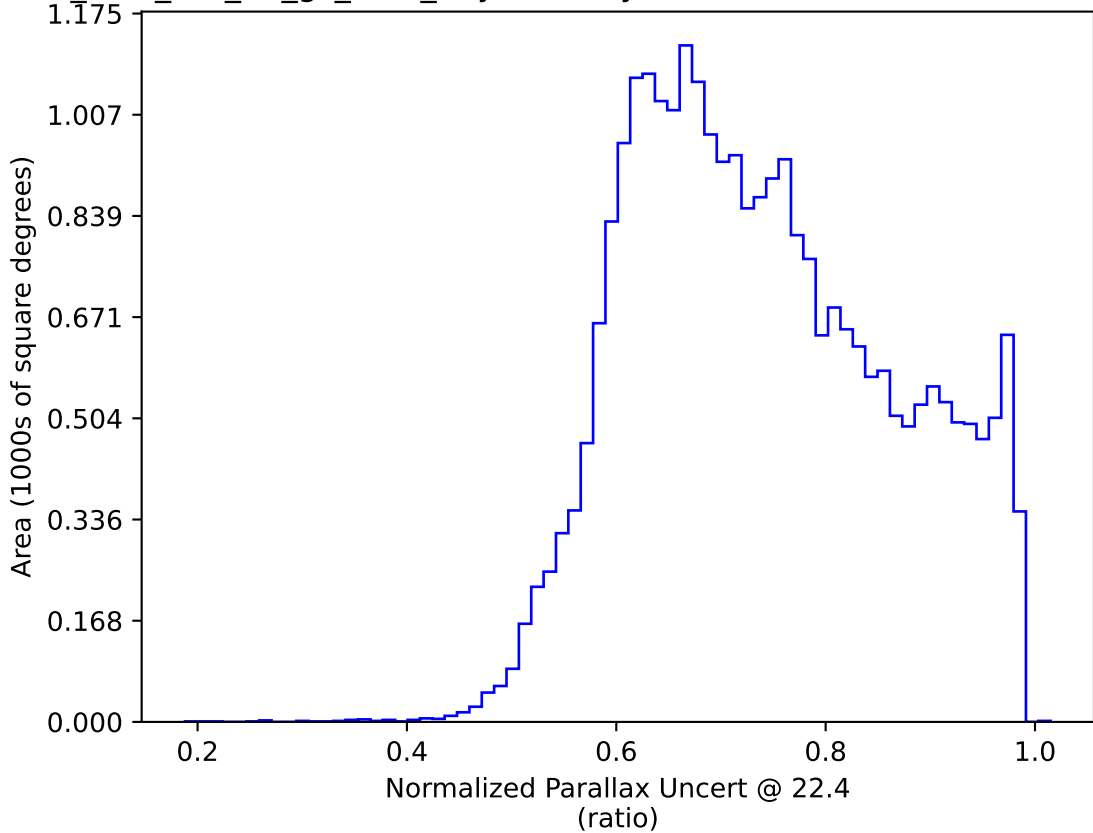
too_elab_r16_d3_gz_v3.4_10yrs All sky: Normalized Parallax Uncert @ 22.4
