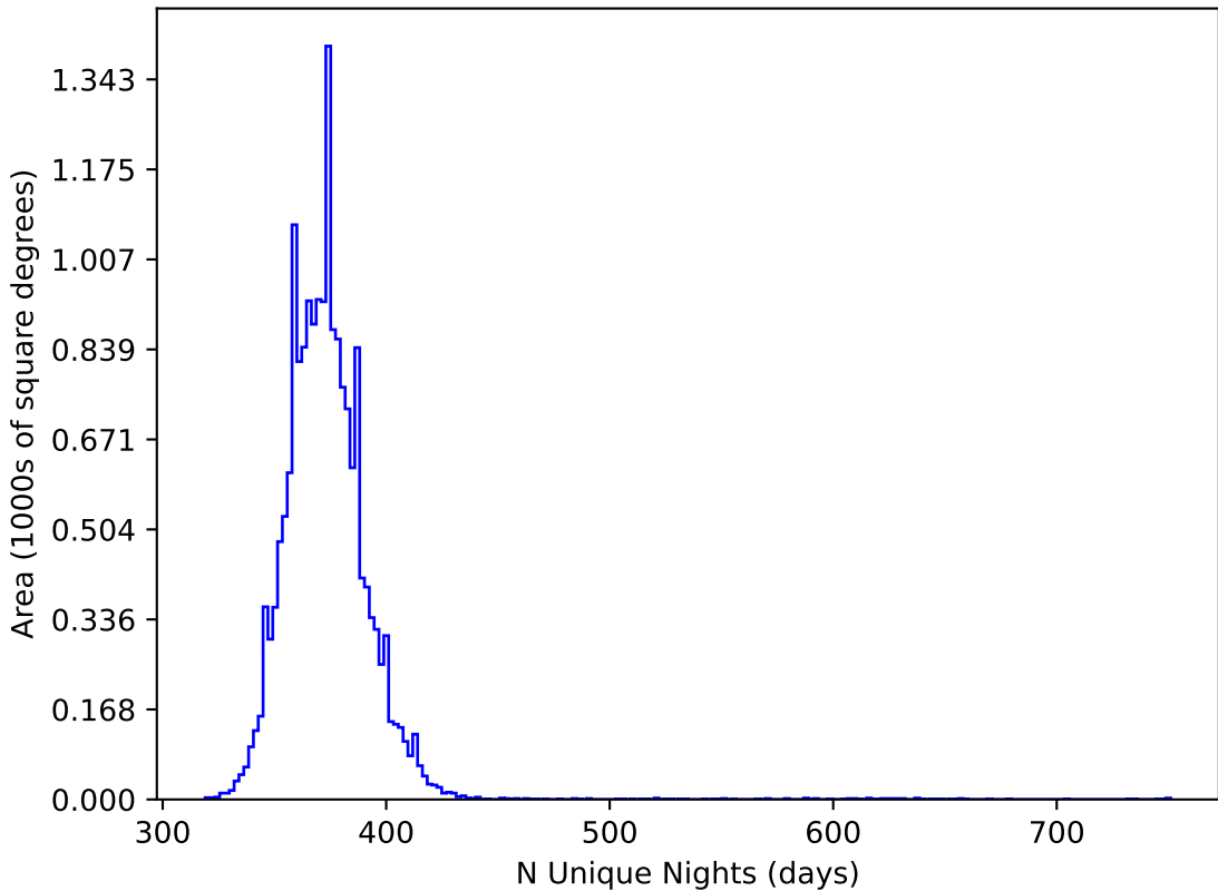
too_elab_r16_d3_gz_v3.4_10yrs WFD all bands: N Unique Nights
