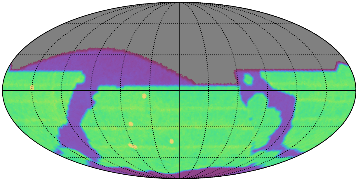
too_elab_r16_d3_gz_v3.4_10yrs All sky all bands: N Unique Nights
