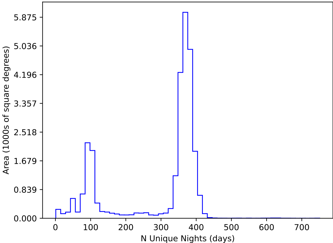
too_elab_r16_d3_gz_v3.4_10yrs All sky all bands: N Unique Nights
