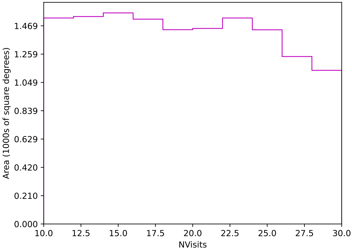
too_elab_r16_d3_gz_v3.4_10yrs Yr 3-4 z band: NVisits
