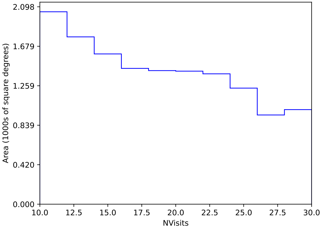
too_elab_r16_d3_gz_v3.4_10yrs Yr 3-4 y band: NVisits
