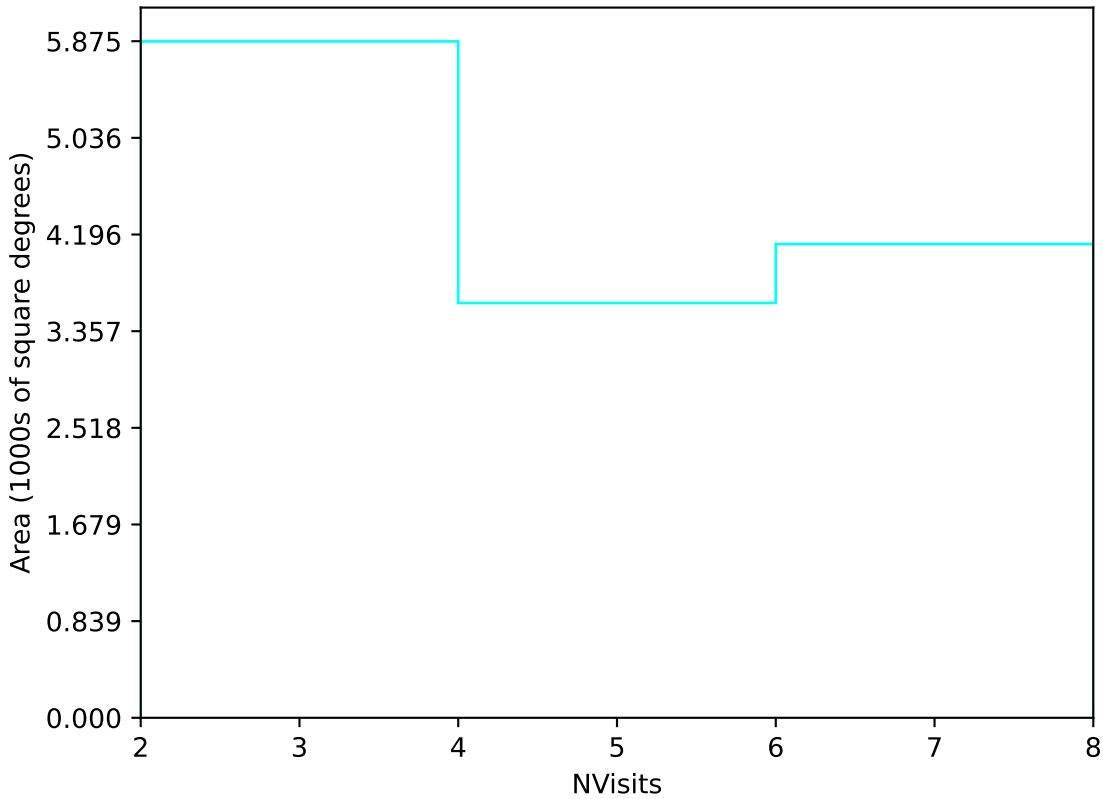
too_elab_r16_d3_gz_v3.4_10yrs Yr 3-4 u band: NVisits
