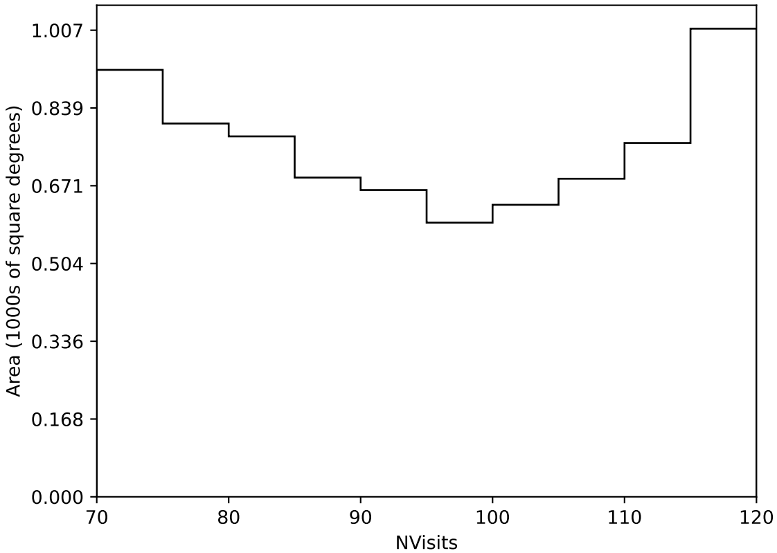
too_elab_r16_d3_gz_v3.4_10yrs Yr 3-4 all bands: NVisits
