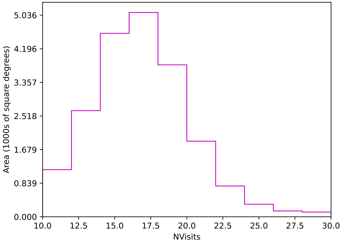
too_elab_r16_d3_gz_v3.4_10yrs Yr 1 z band: NVisits
