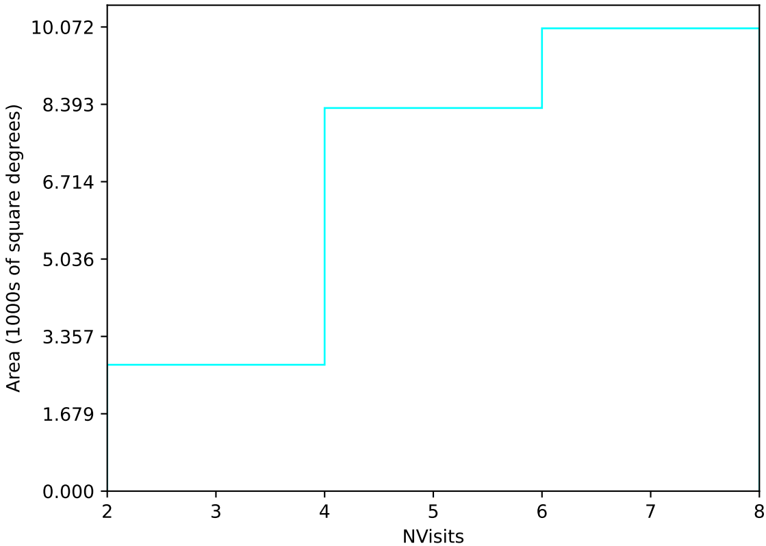
too_elab_r16_d3_gz_v3.4_10yrs Yr 1 u band: NVisits
