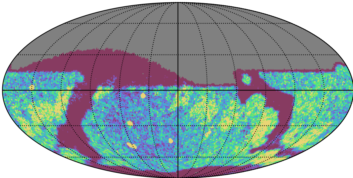
too_elab_r16_d3_gz_v3.4_10yrs Yr 1 r band: NVisits
