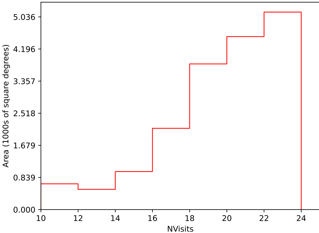
too_elab_r16_d3_gz_v3.4_10yrs Yr 1 i band: NVisits
