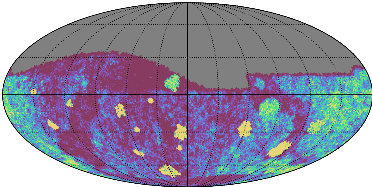
too_elab_r16_d3_gz_v3.4_10yrs Yr 1 g band: NVisits
