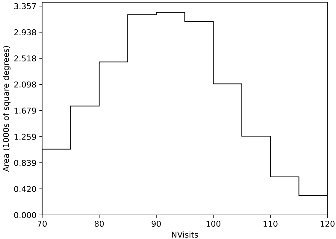
too_elab_r16_d3_gz_v3.4_10yrs Yr 1 all bands: NVisits
