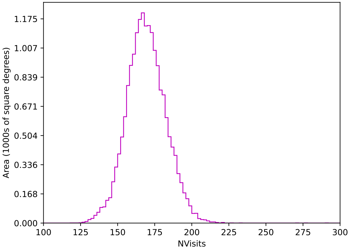
too_elab_r16_d3_gz_v3.4_10yrs WFD z band: NVisits
