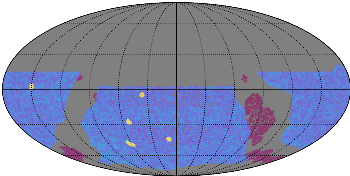
too_elab_r16_d3_gz_v3.4_10yrs WFD y band: NVisits
