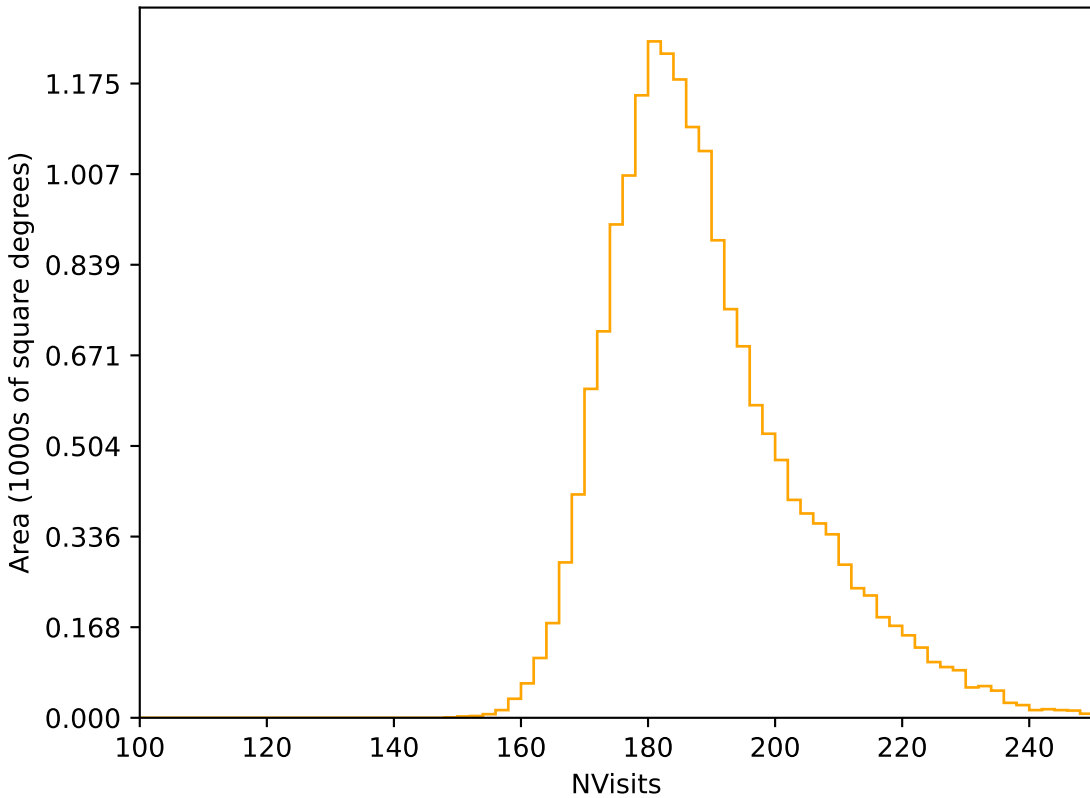
too_elab_r16_d3_gz_v3.4_10yrs WFD r band: NVisits
