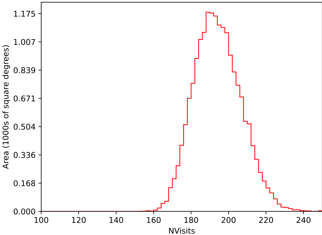
too_elab_r16_d3_gz_v3.4_10yrs WFD i band: NVisits
