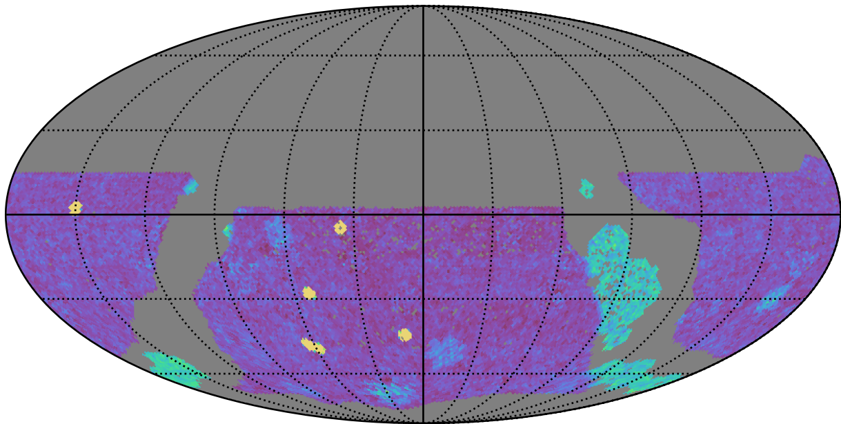
too_elab_r16_d3_gz_v3.4_10yrs WFD g band: NVisits
