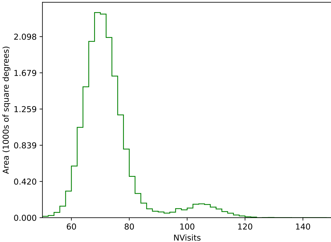
too_elab_r16_d3_gz_v3.4_10yrs WFD g band: NVisits
