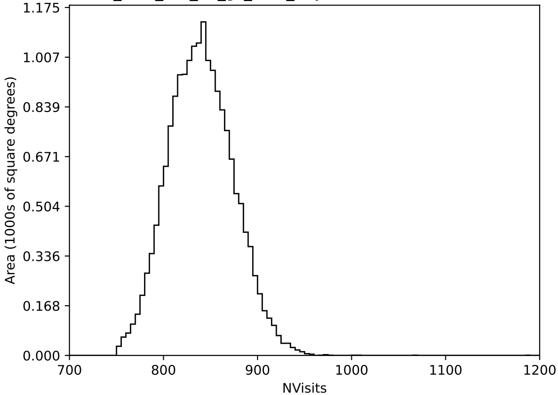
too_elab_r16_d3_gz_v3.4_10yrs WFD all bands: NVisits
